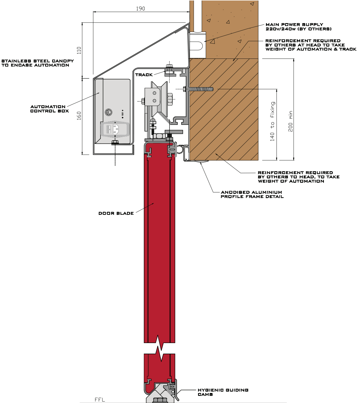
Side section, DT-04 automation with canopy
