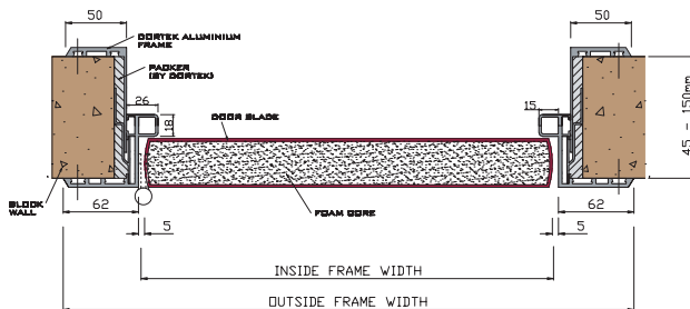
Left hand hung blade illustrated, fixed to aluminium frame on blockwork wall
